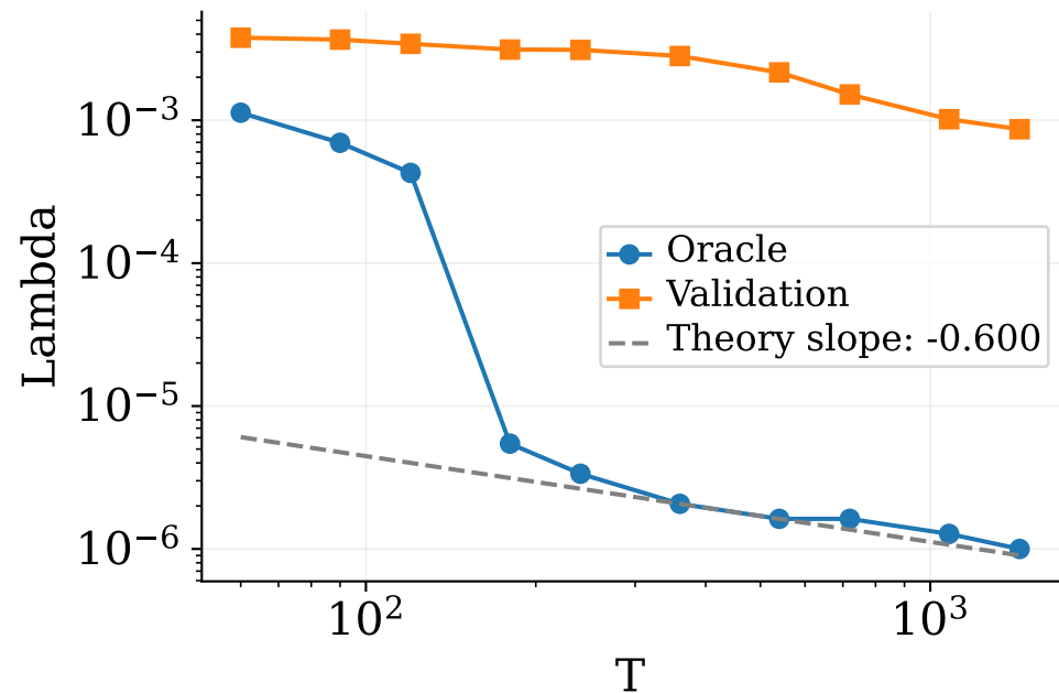
Monte Carlo rate paths and theoretical slopes
